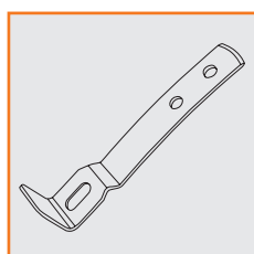
SHOP-NR. 11176 ITEM NO. 7418 Sonderwinkel VELO 42 + 47 Angle VELO 42 + 47
